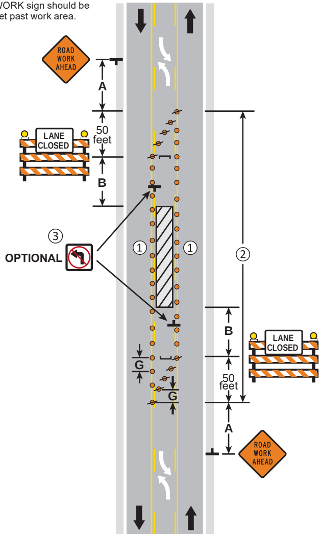
TURN LANE CLOSURE TWO-WAY CONTINUOUS LEFT-TURN LANE 3 DAYS or LESS
