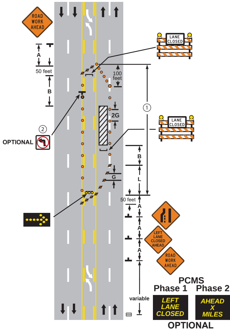
LEFT LANE CLOSURE - 5 LANE SECTION TWO-WAY CONTINUOUS LEFT-TURN LANE 3 DAYS or LESS
